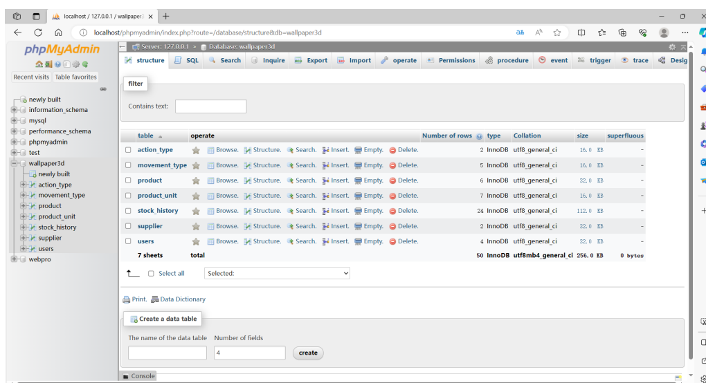
Figure 2.2 MySQL Database [2]
