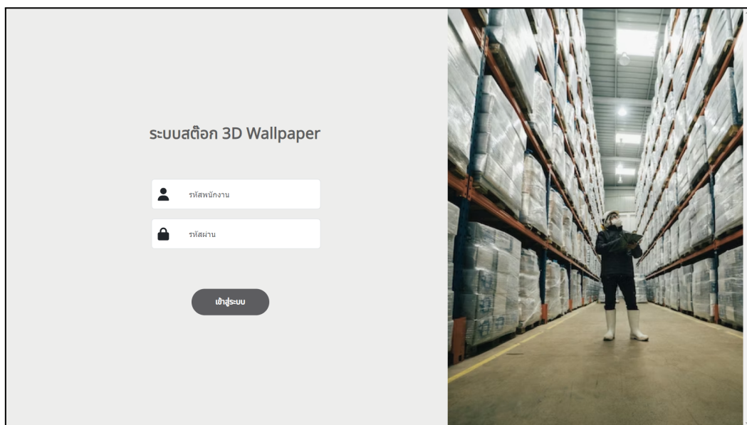
Figure 4.1 Login page
